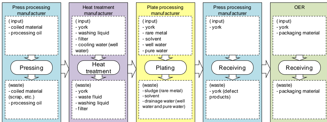
Figure 31.1 Input/output in each quantity center
