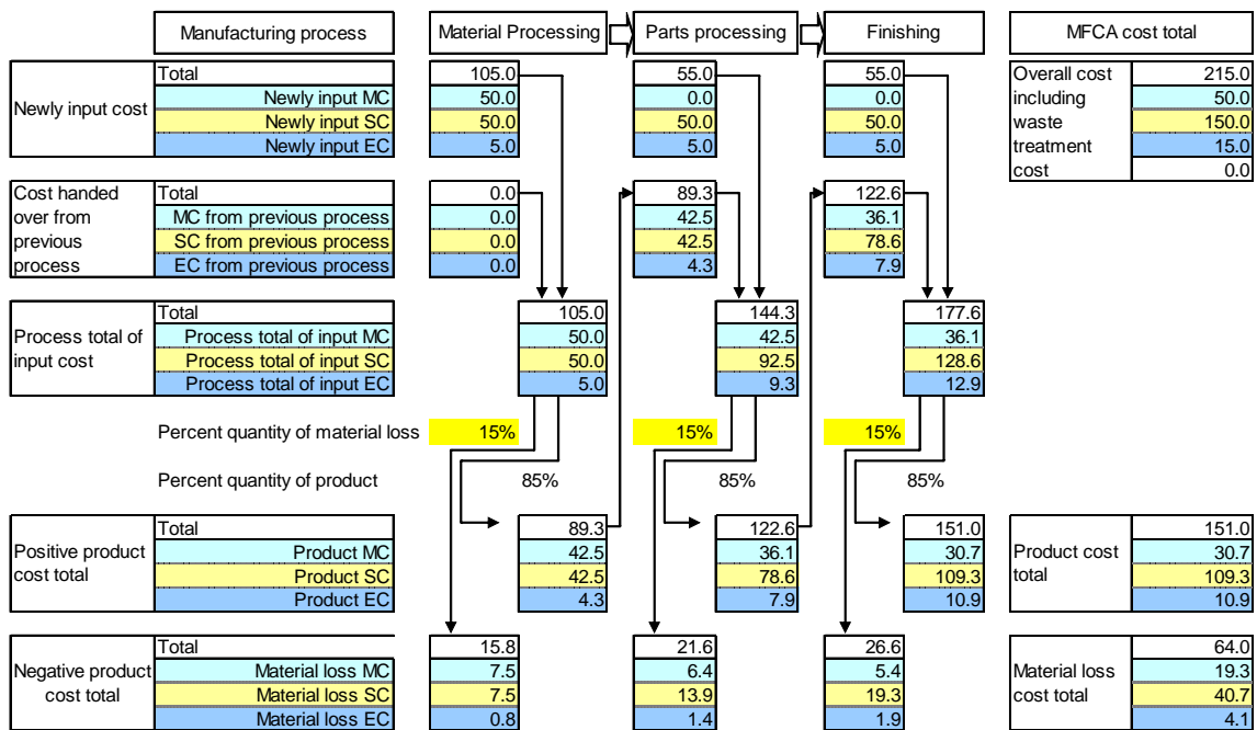
Figure V-4 Example calculation by simplified MFCA trial tool
