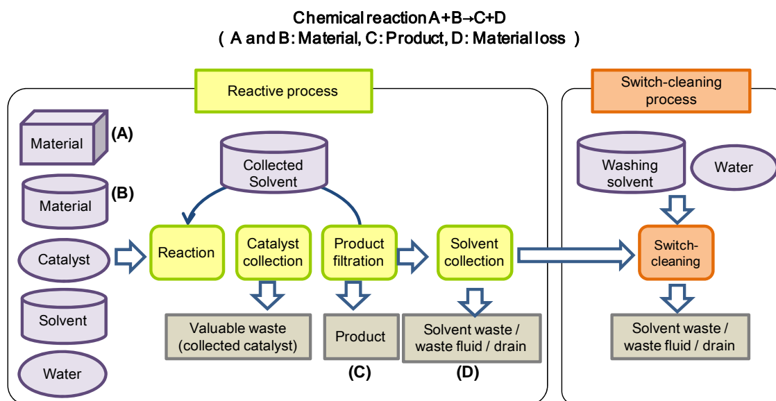
Figure 5.1 Input/output of each quantity centre
