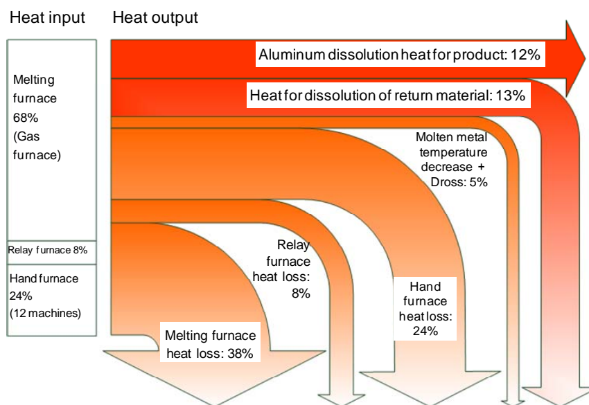
Figure 13.4 Heat calculation result for line that involves concentration melting furnace
