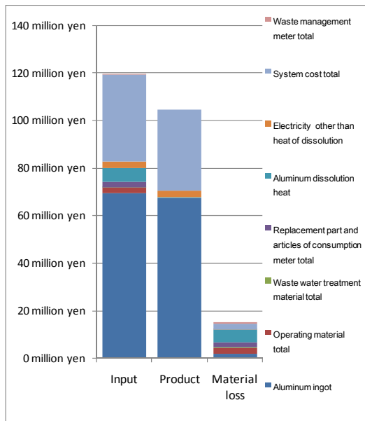
Figure 13.2 MFCAs calculation result
